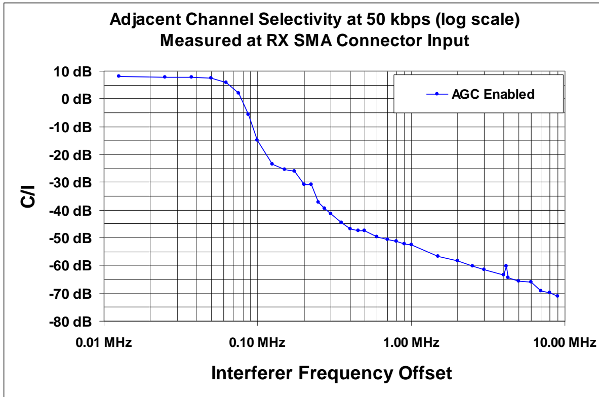
Figure 45. Receiver Selectivity
